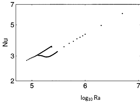
FIG. 1. The Nusselt number for convecting flows of various Rayleigh numbers. Within the hysteretic range, two flow morphologies are possible, each corresponding to a different Rayleigh number. For example, at Ra=2 \times 10^5 , a harmonic flow with Nu=3.392 and a chaotic flow with Nu=2.959 are both stable possibilities.
